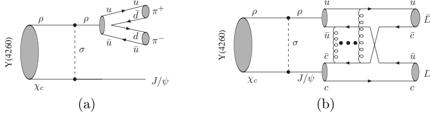
Figure 1: (a) and (b) correspond to Y(4260) \rightarrow J/\psi\pi^+\pi^- and the Y(4260) \rightarrow D\bar{D} decays respectively.
