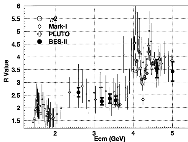
FIG. 2. Plot of R values vs E_{\text{cm}} . The R values from BES are taken from Table I with an error which combines statistical and systematic errors quadratically.
